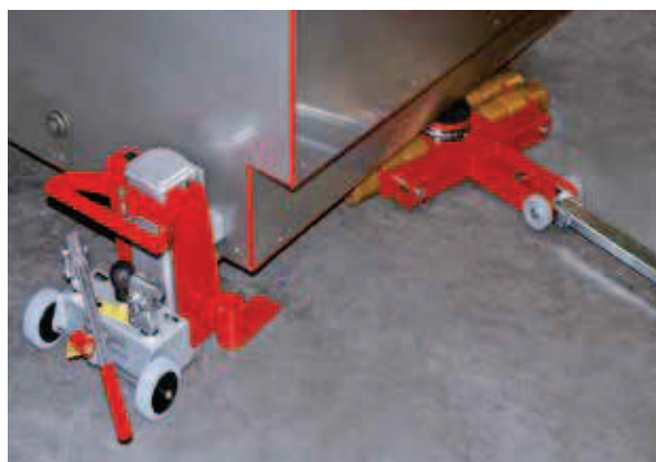
JH 15 G plus in use combined with our JL 9 K
